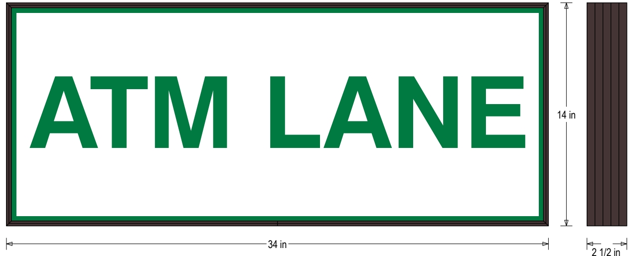
Frame Detail
