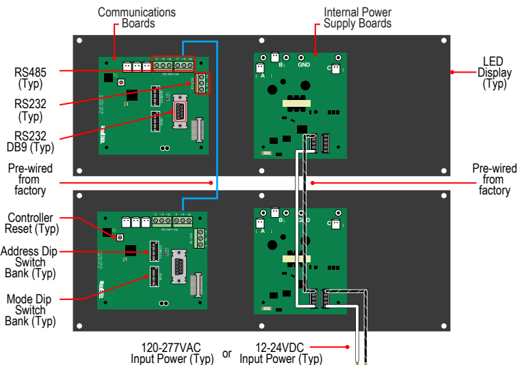
Fig. 2: Wiring a 120-277VAC Power Supply
