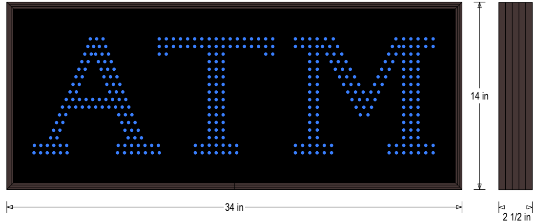
Frame Detail
