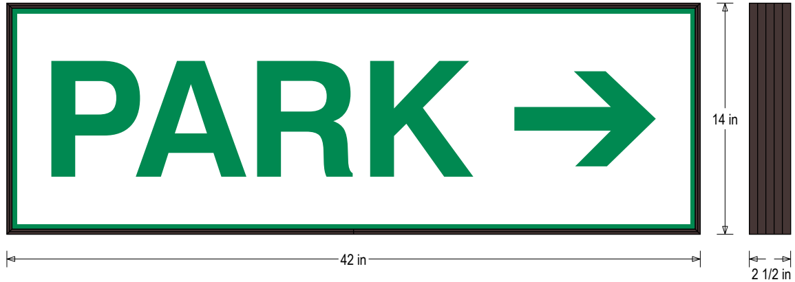
Frame Detail
