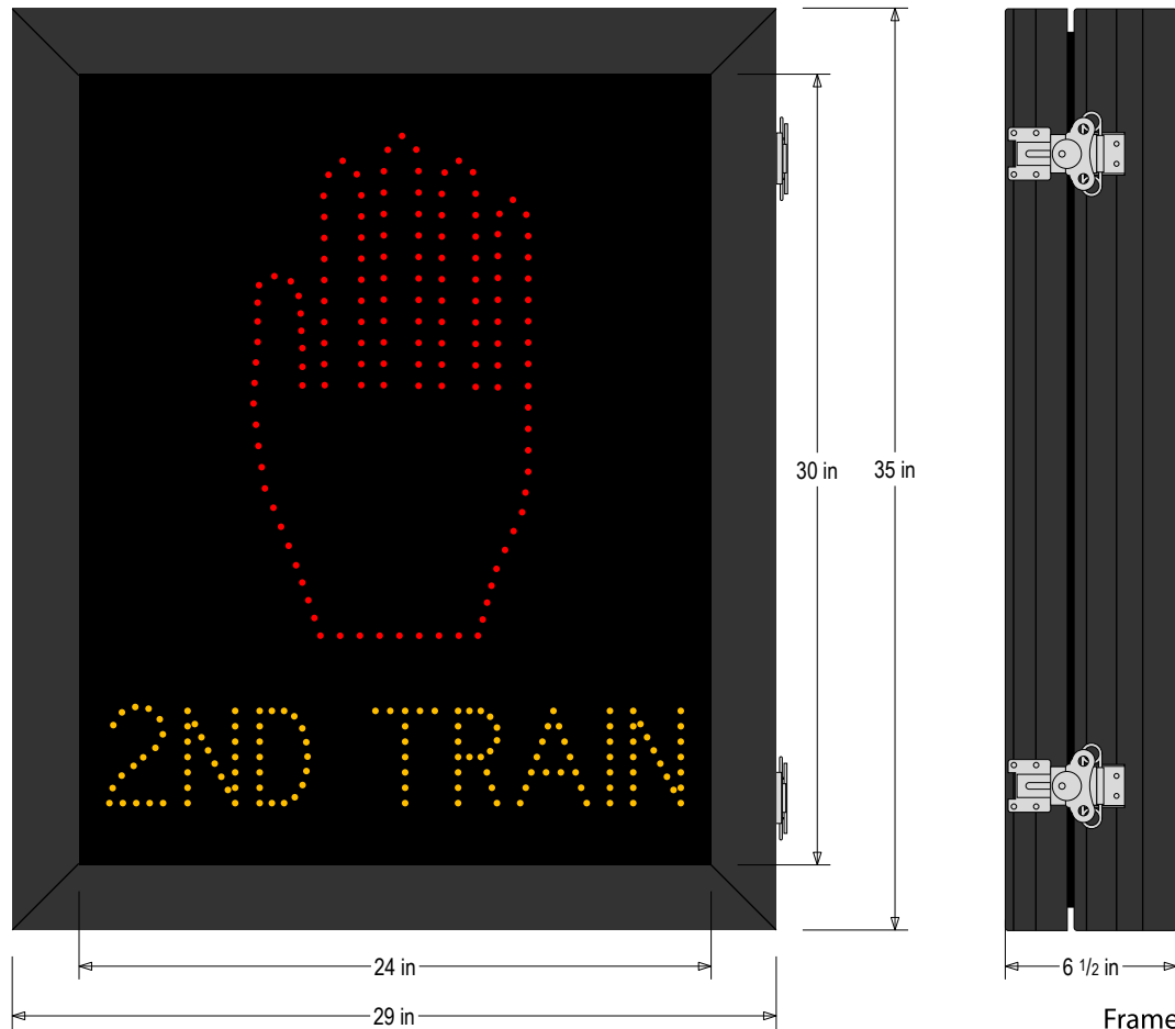
Frame Detail
