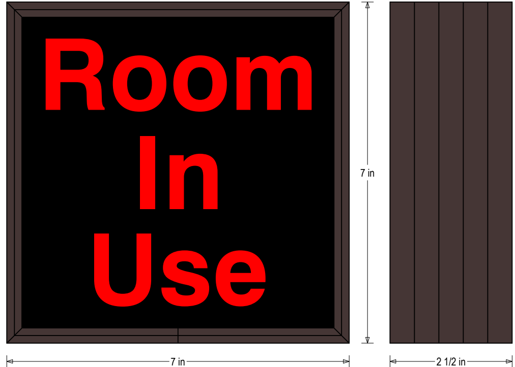
Frame Detail
