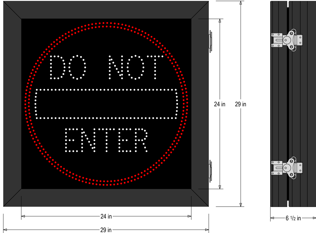
Frame Detail
