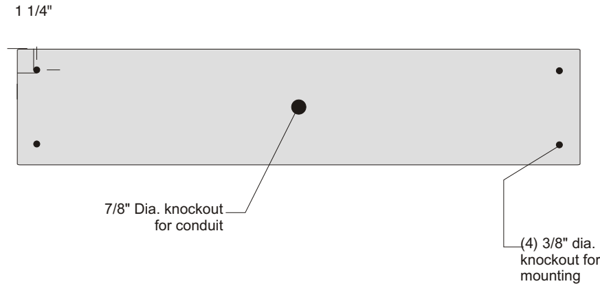
Back View
