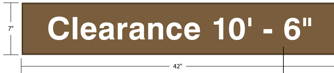
Front View
