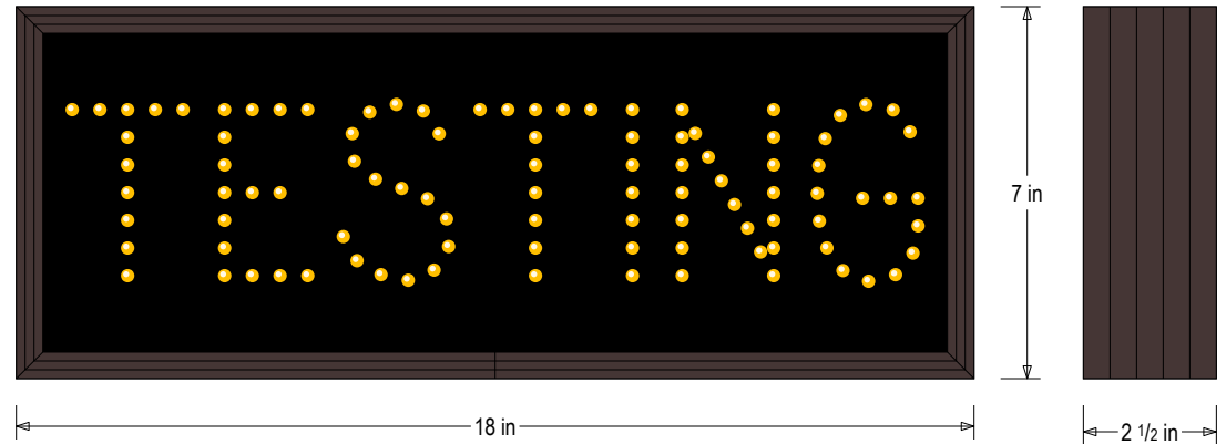
Frame Detail
