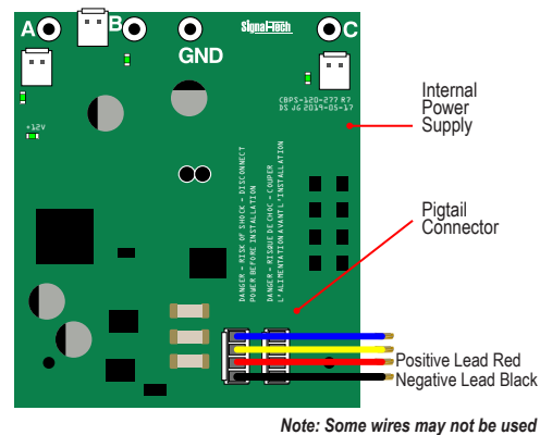
Fig. 3: Wiring a 12-24VDC Power Supply
