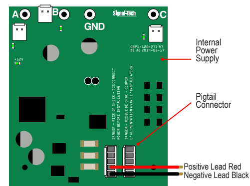
Fig. 2: Wiring a 12-24VDC Power Supply
