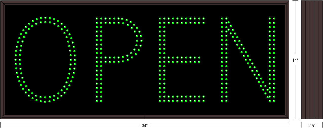
Frame Detail
