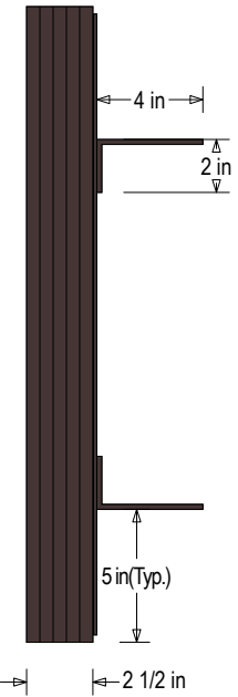
1/8" Back w/ 2 (two) 2"x4" Angle Mounts
