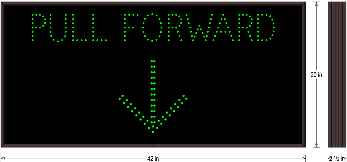
Frame Detail
