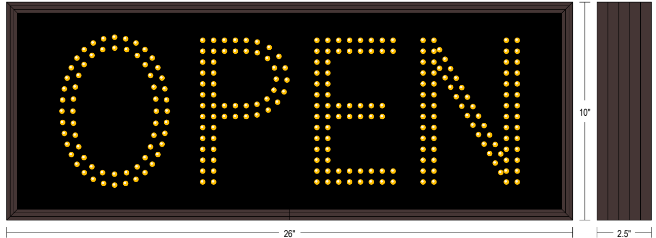
Frame Detail
