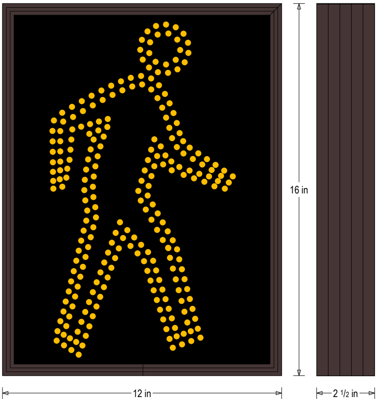
Frame Detail
