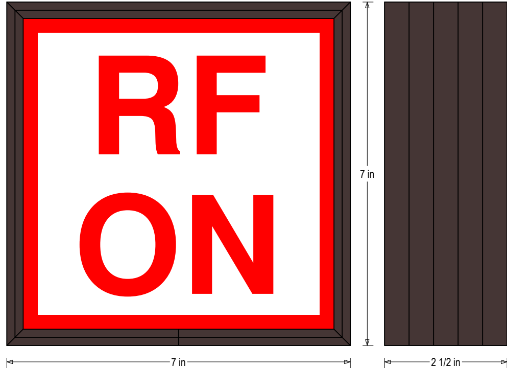
Frame Detail
