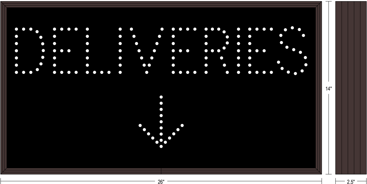
Frame Detail
