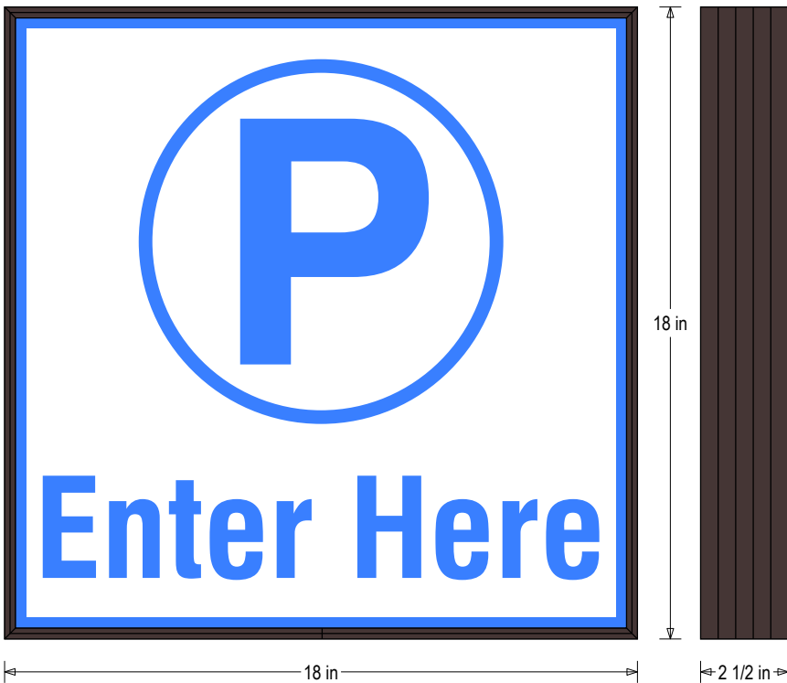
Frame Detail
