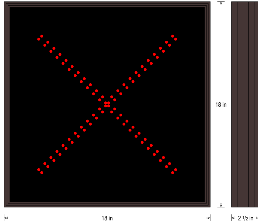
Frame Detail
