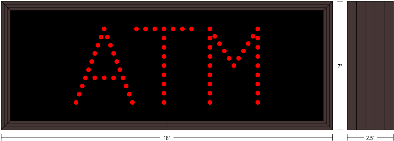
Frame Detail
