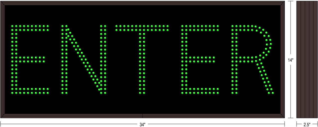
Frame Detail
