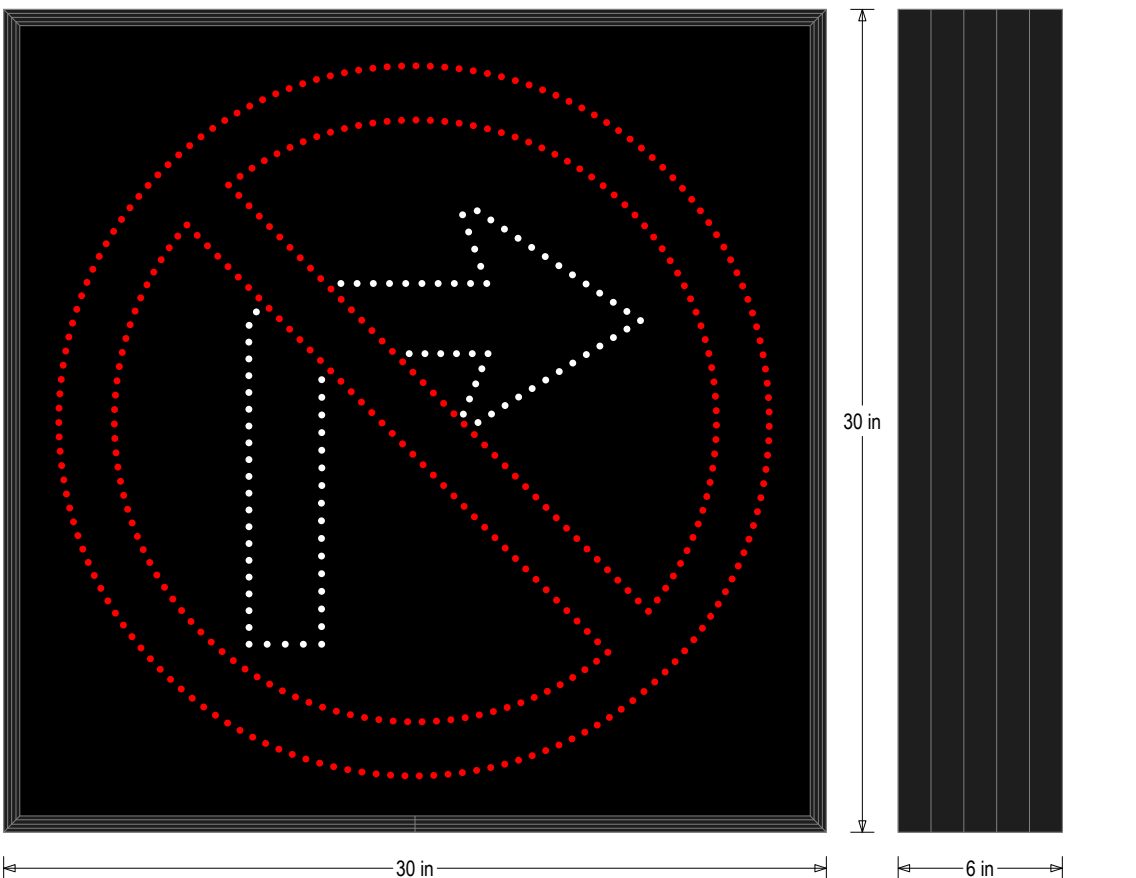
Frame Detail
