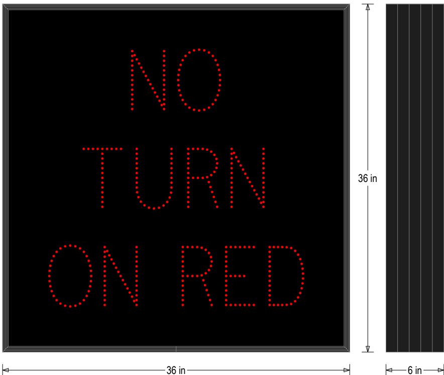
Frame Detail
