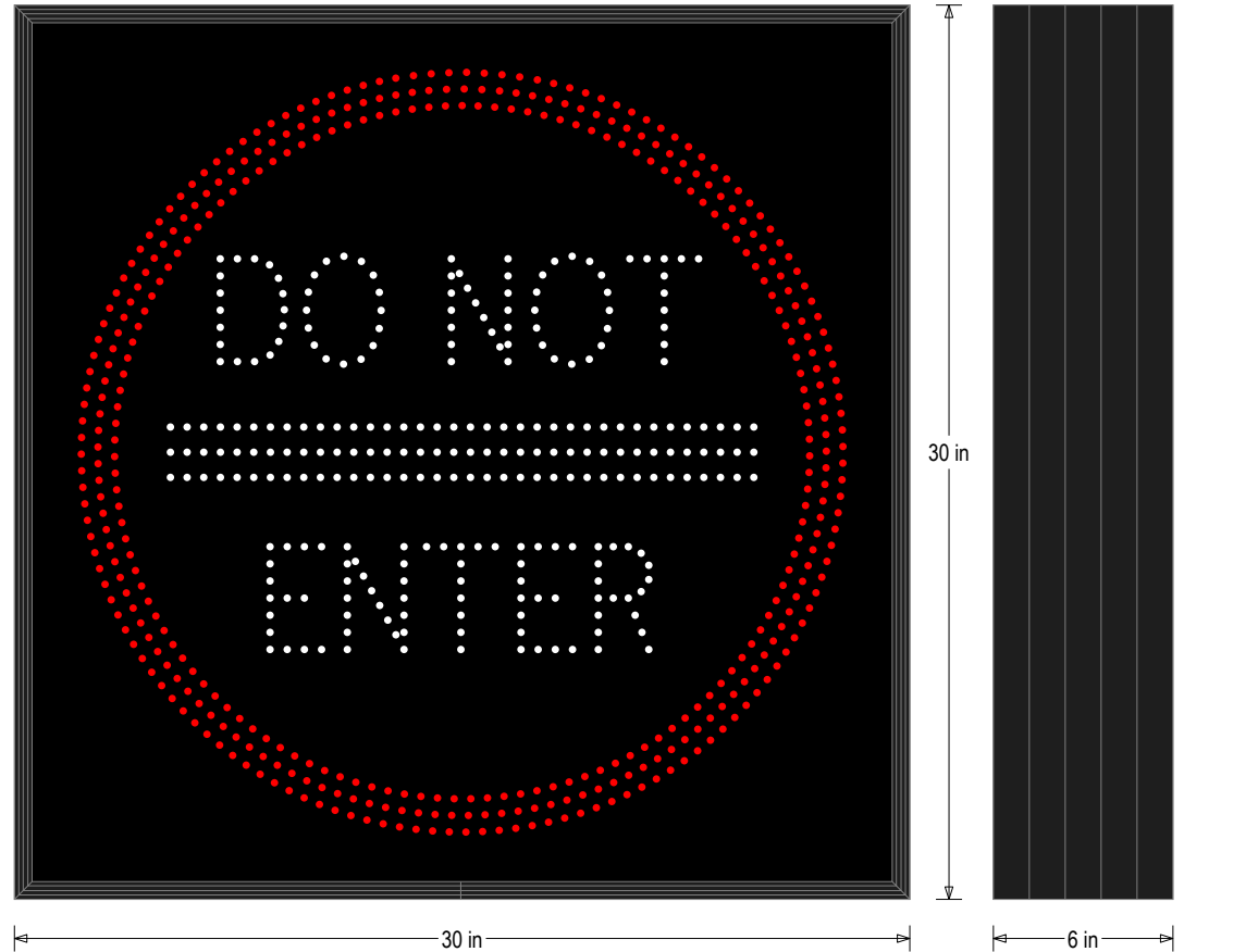
Frame Detail
