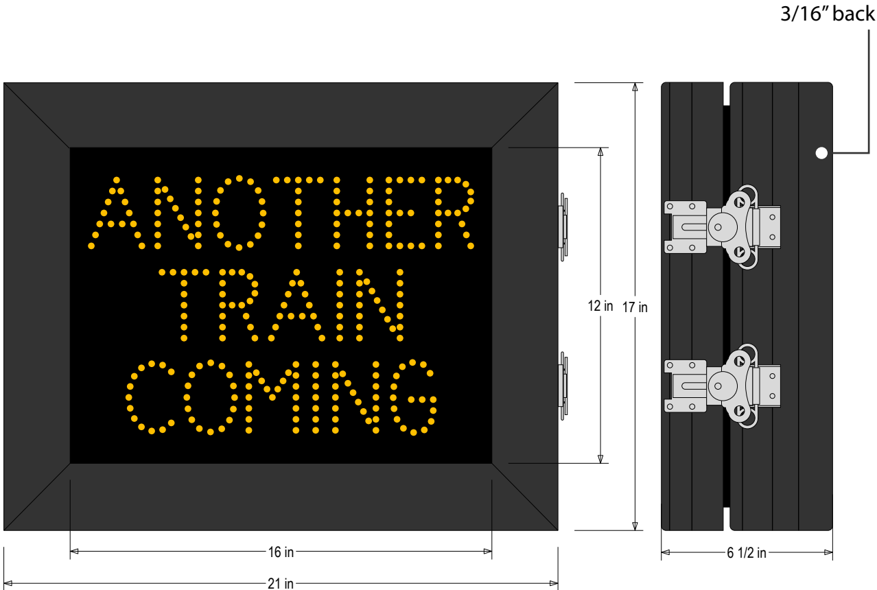
Frame Detail
