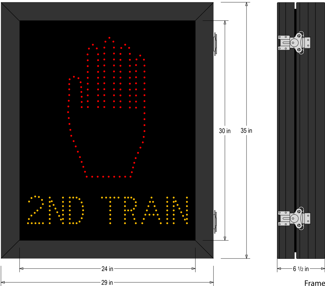
Frame Detail
