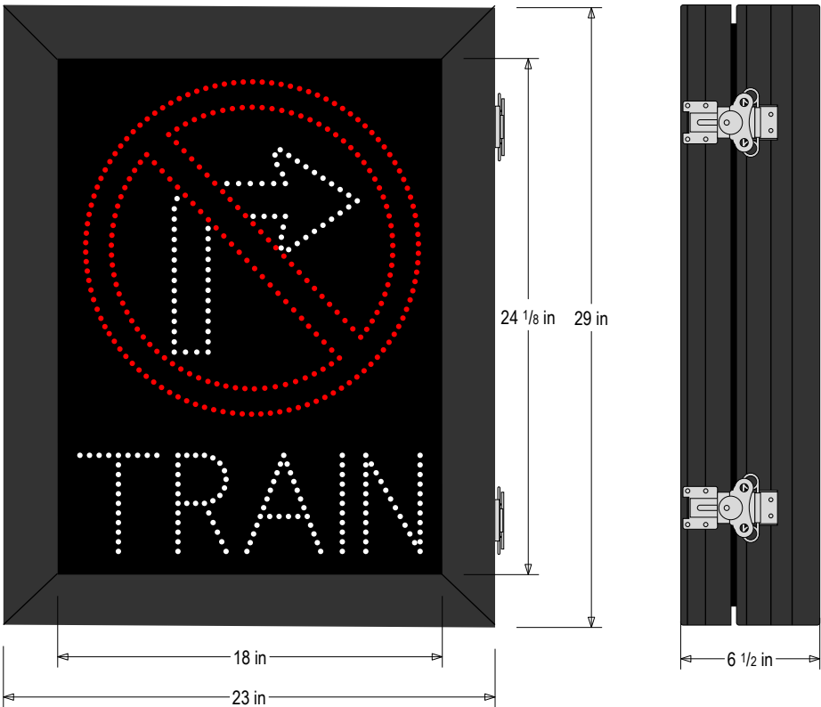
Frame Detail
