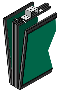
Frame Detail
