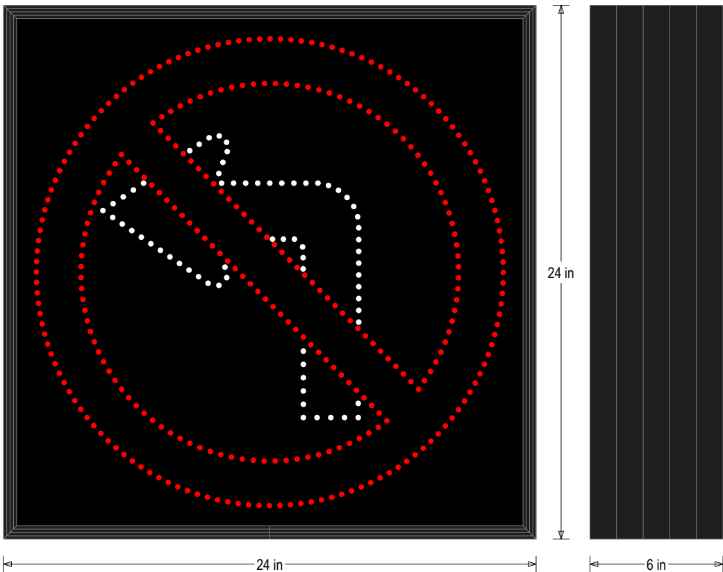
Frame Detail
